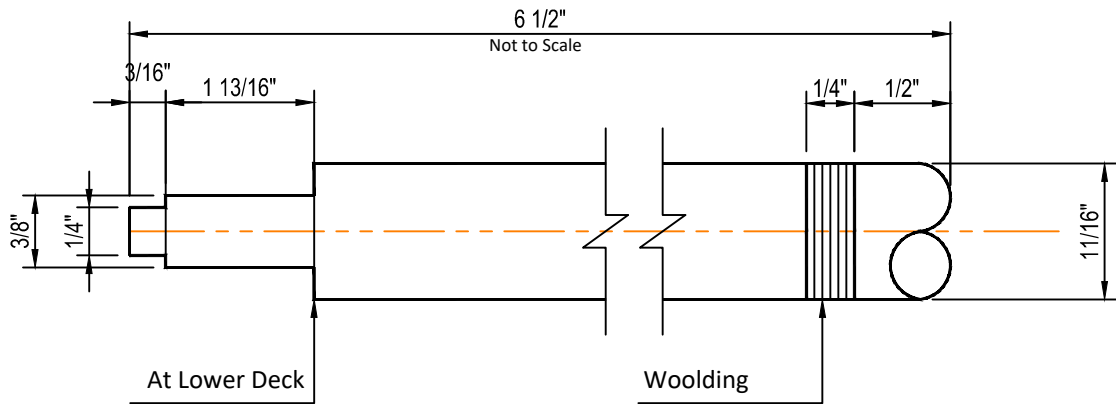
Main Mast
